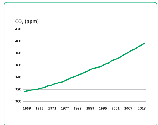
Figure 12.10 Growth in emissions results in high levels of CO 2 in the atmosphere
