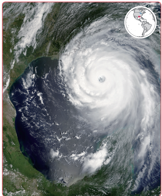
Figure 1.2 Hurricane Katrina
