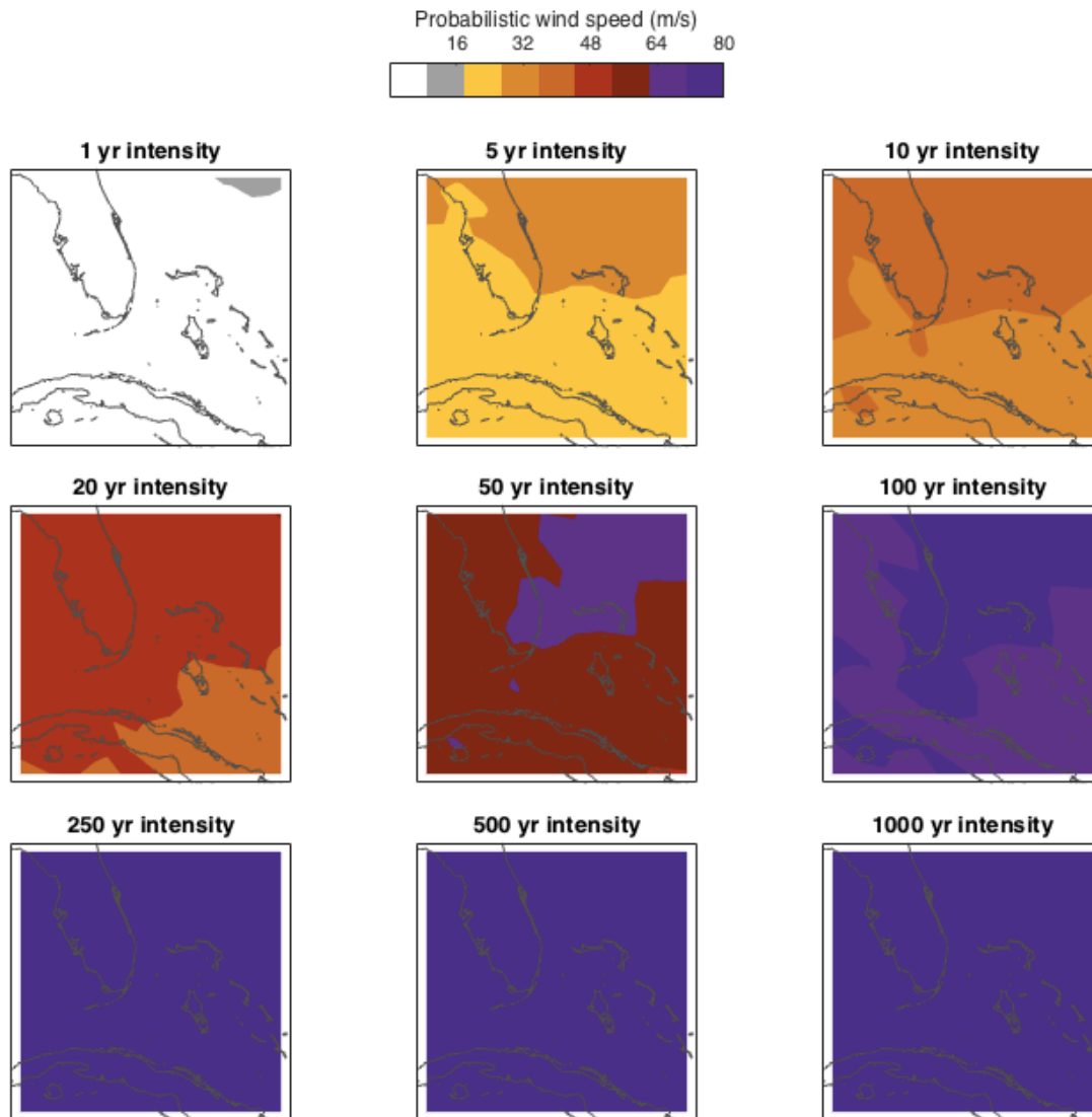
Figure: climada_hazard_stats(hazard);
